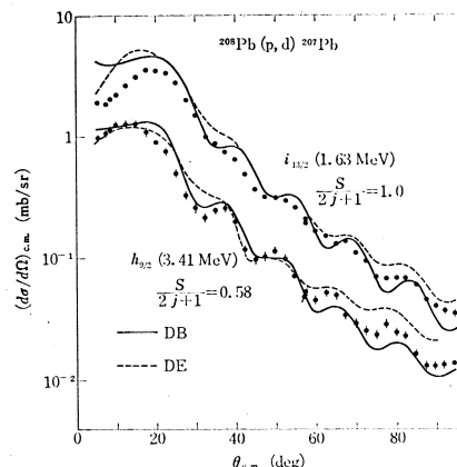
Fig. 3 (c) Differential cross sections of the ^{208}\text{Pb}(p, d)^{207}\text{Pb} at E_p=52 MeV. Solid curves are due to the DB analysis and broken curves to the DE analysis. The r_{0n}=1.25 fm is used.
